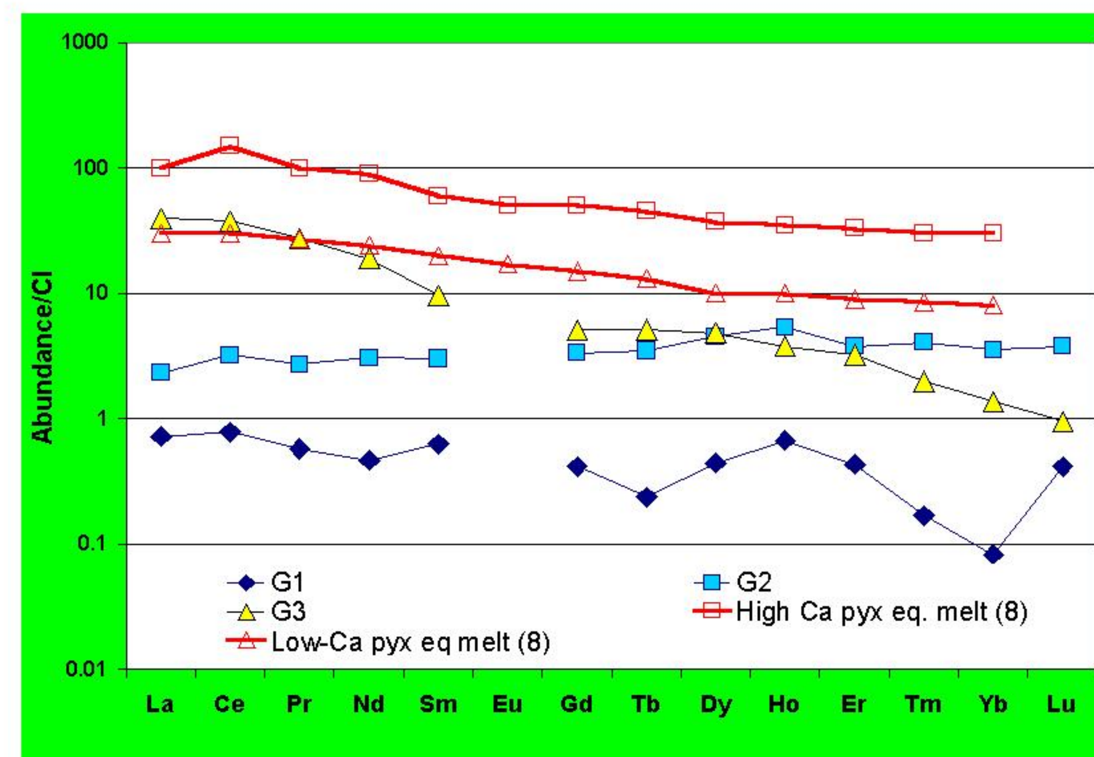
Fig.2b: REE abundances of glasses: G1, G2 and G3. Calculated melt in equilibrium with early and late phases [8] are given for comparison.
