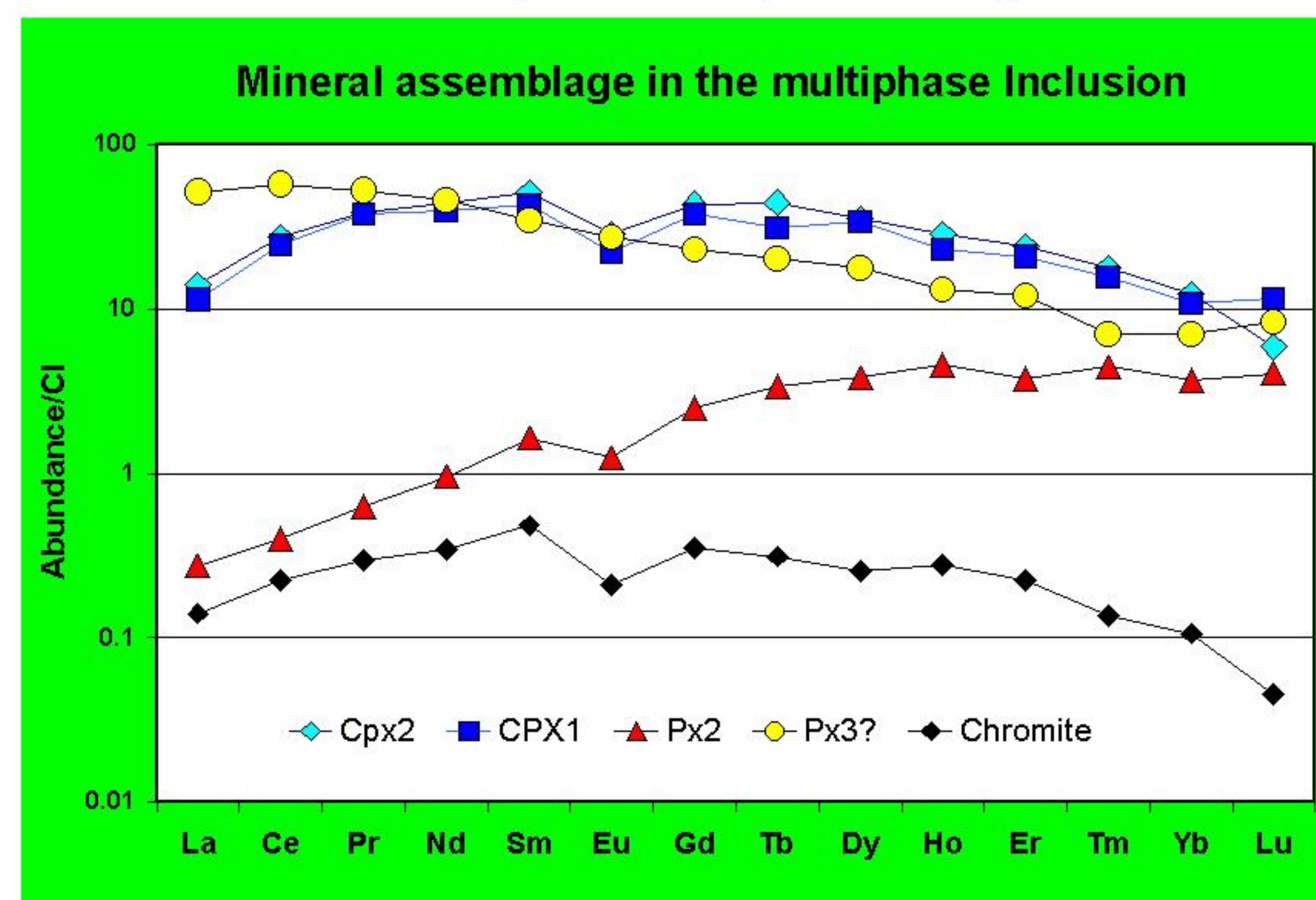
Fig.2 a: REE abundances of the mineral assemblage in the multiphase inclusion
