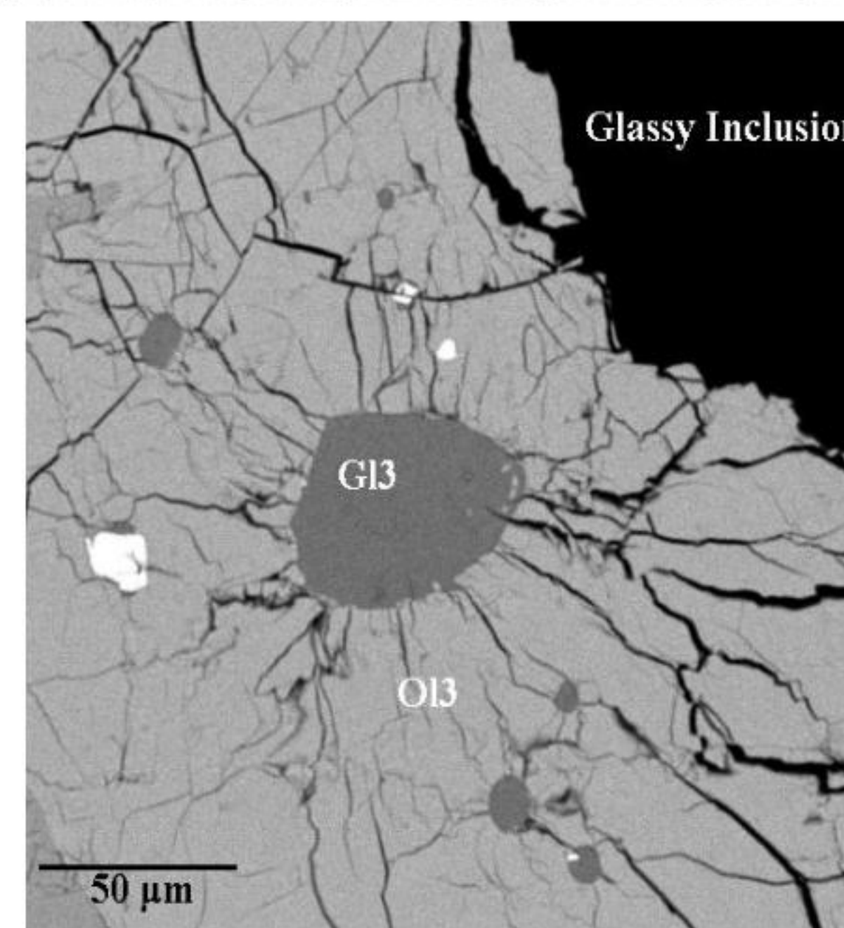
Fig. 1: BSE images of the multiphase and glassy inclusion in Chassigny L6101.
