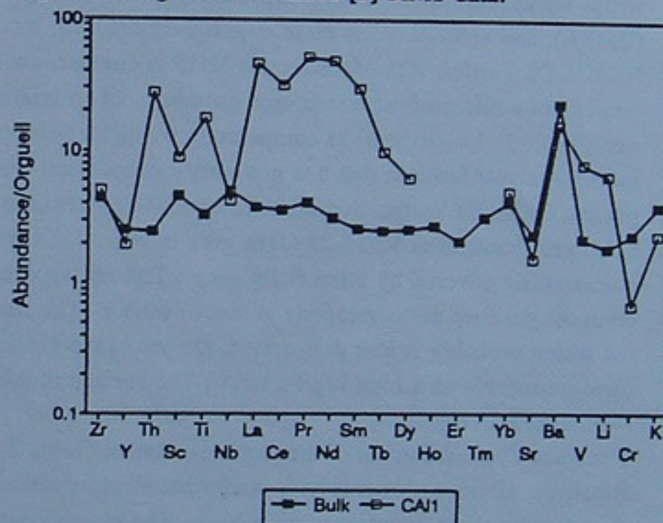
Figure 2: Orgueil-normalized [3] SIMS data.
