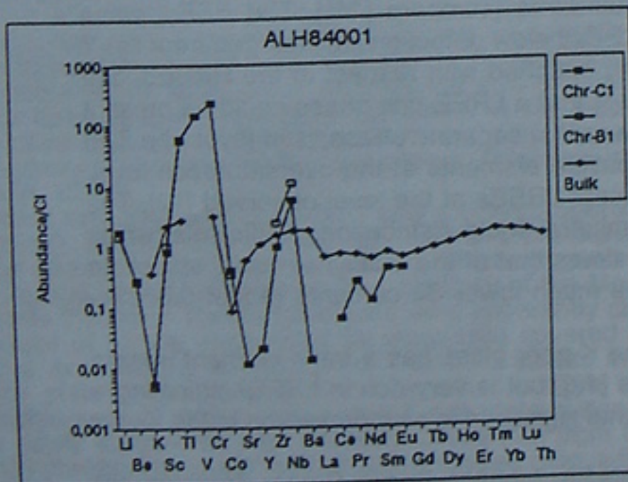
Figure 3: CI-normalized elemental abundances in large chromite (Fig. 2) compared to ALH84001 bulk composition [6].
