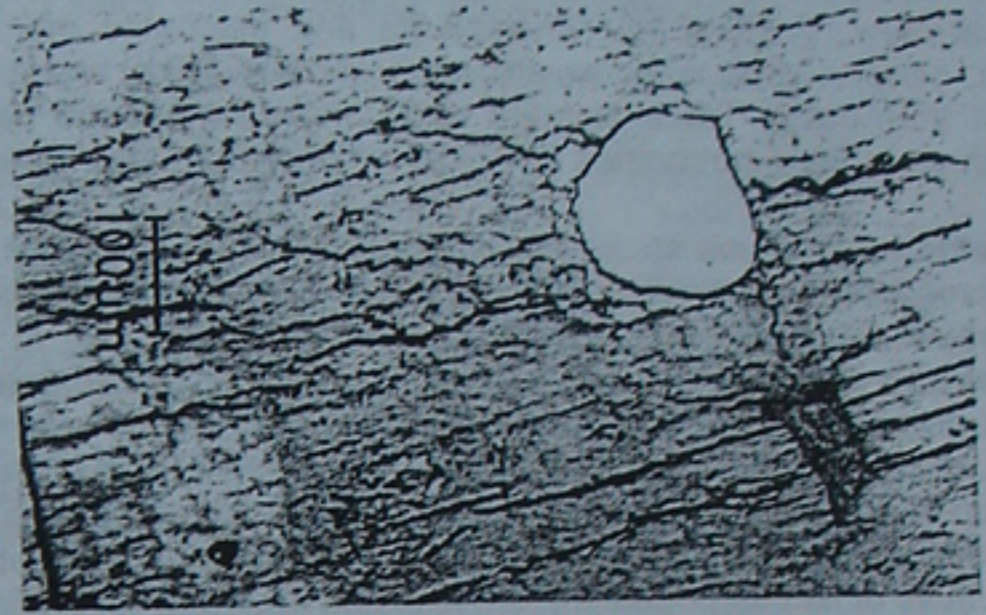
Figure 2: Large chromite and granular chromite (light grey) enclosed in orthopyroxene with adjacent angular pocket of feldspar-like glass (dark grey) which also contains K-rich glass and silica. Optical micrograph, reflected light.
