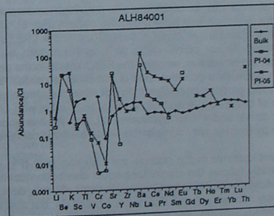
Figure 4: CI-normalized elemental abundances in a K-poor (PI-4) and K-rich (PI-5) glass compared to ALH84001 bulk composition [6].
